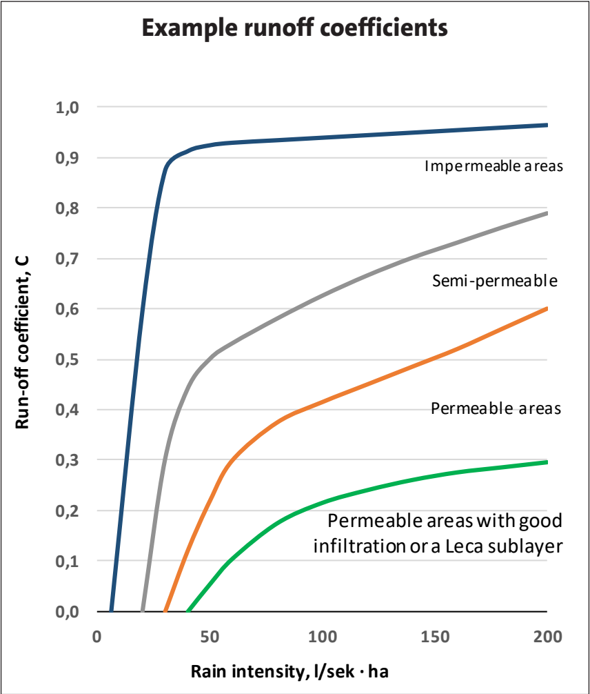
Examples of development of runoff coefficients (C) for different surfaces with increasing rain intensity. The permeable surface, combined a Leca LWA subsurface layer, will resist increase in runoff, even at high rain intensities.
